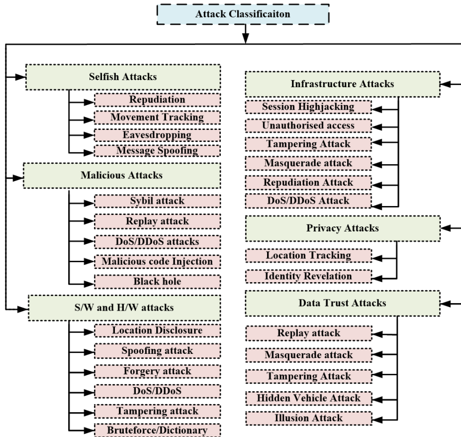
FIGURE 4. Attacks classification for V2X environment [83]
