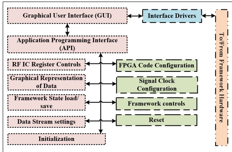
FIGURE 3. A generic IoT-V2X software structure [58]
